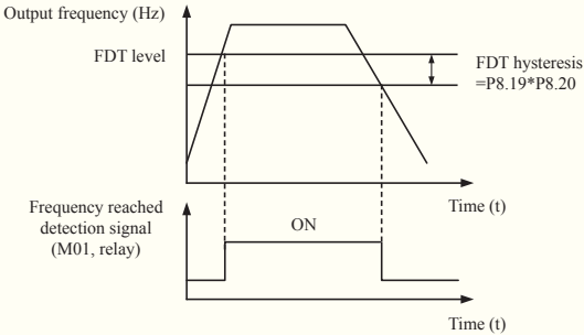
Figure 4-14 FDT level
